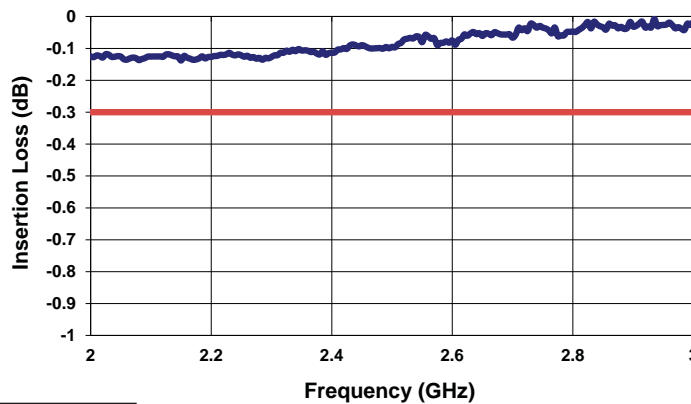
Insertion Loss ( 2-3 GHz )
