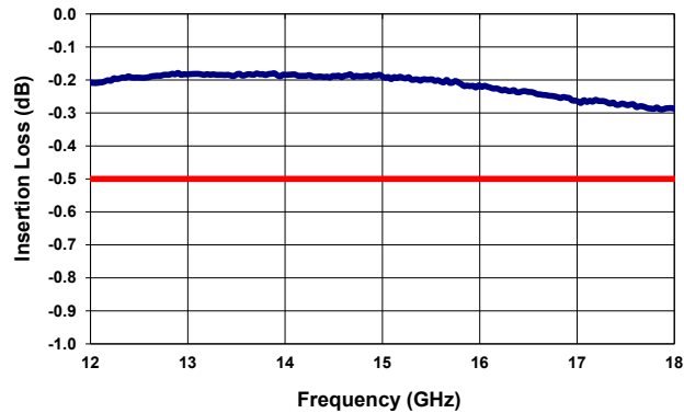
Insertion Loss ( 12-18 GHz )
