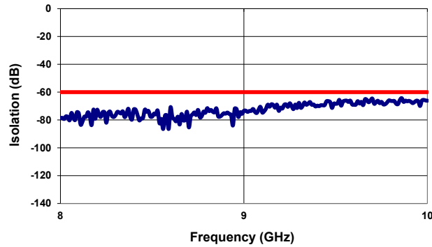
Isolation ( 8-10 GHz )
