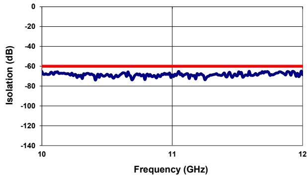
Isolation ( 10-12 GHz )
