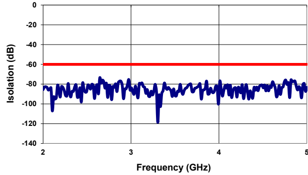
Isolation ( 2-5 GHz )
