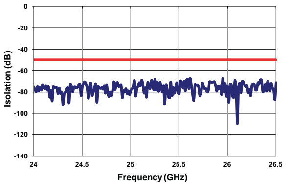
Isolation (24-26.5 GHz)
